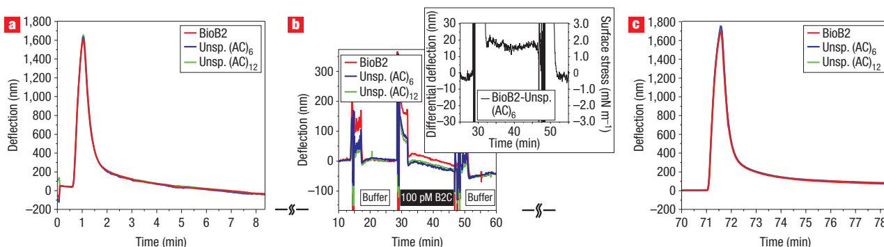
Figure 2 Calibration of the mechanical response and the biosensitivity of the cantilever array sensors. a,b , Calibration by application of a heat pulse of 0.7 °C for 30 s ( a ), followed by 100 pM complementary BioB2 cDNA injection ( b ), which results in compressive stress due to hybridization of the specific complementary cDNA with an absolute signal of ~17 nm. Inset: The differential signal is evaluated by subtracting the response of the Unsp. (AC) 6 -sensitized cantilever from the signal of the BioB2-sensitized cantilever. c , Cantilever sensor calibration by applying a heat pulse after the sensitivity-validation experiment. This demonstrates the mechanical stability and integrity of the sensors.
