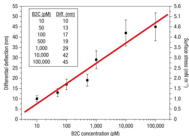
Figure 4 Differential nanomechanical response of cantilevers during specific hybridization. Compressive stress response versus concentration dependence. The error bars represent standard deviation obtained from four measurements.
