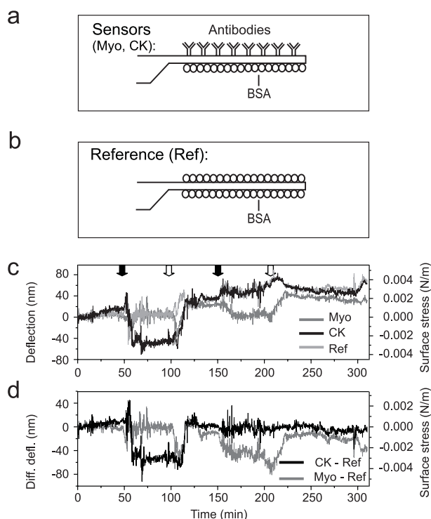
Figure 4. (a) Two cantilevers in the array are coated with myoglobin (Myo) and creatin kinase (CK) antibodies and passivated on their lower surface with BSA. (b) The reference cantilever is quenched on the two surfaces with BSA. (c) Sequential injections of creatin kinase and myoglobin proteins reveal deflection of the corresponding cantilever due to compressive stress. The experiment is performed in a background of unspecific protein (BSA 100 \mu\text{g ml}^{-1} ). (d) Differential deflection signals: CK-Ref, Myo-Ref.
