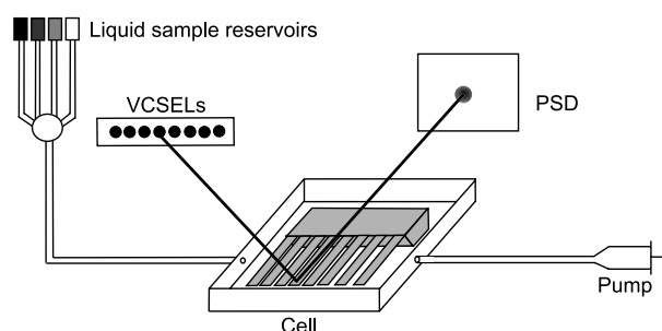
Figure 1. Schematic of the experimental setup with liquid cell, optical readout of cantilever deflections and sample liquid exchange system. VCSEL = vertical cavity surface emitting lasers, PSD = position sensitive detector.
