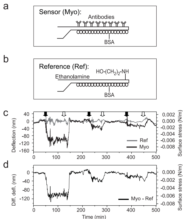
Figure 3. (a) The sensor cantilever is functionalized with myoglobin (Myo) antibodies and the lower surface is passivated with BSA. (b) The reference cantilever is quenched on the upper surface with ethanolamine, and the lower surface is passivated with BSA. (c) Myoglobin (Myo) was detected at three different concentrations ( 100, 50, 20 \mu\text{g ml}^{-1} ). The reference cantilever (Ref) does not show a significant response. (d) Differential deflection signal (Myo–Ref): the response of the sensor cantilever is almost linear with protein concentration in the range investigated. The accuracy of deflection determination is 20%, as derived from the noise in the cantilever deflection divided by deflection magnitude.
