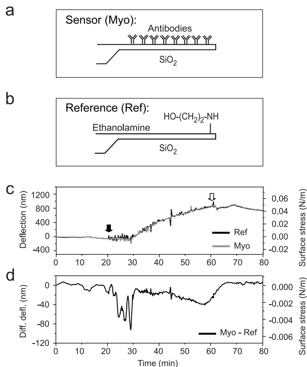
Figure 2. (a) Sensor cantilever functionalized with myoglobin (Myo) antibodies, (b) reference cantilever (Ref) quenched with ethanolamine. The lower surfaces are not passivated. (c) Absolute deflection of cantilevers. Upward bending of the cantilever increases deflection and produces tensile surface stress, whereas downward bending of the cantilever decreases deflection and builds up compressive surface stress. Myo is shown in black, Ref in grey. The black arrow indicates protein injection, white arrows injection of buffer. The injection of myoglobin protein ( 50 \mu\text{g ml}^{-1} ) produces drift of both cantilevers. No conclusive interpretation is possible owing to the competition between unspecific interaction of protein with lower silicon surface of the cantilevers and antigen–antibody interaction on the upper surface. (d) Differential deflection signal (Myo–Ref). The net reaction response is 40 nm.
