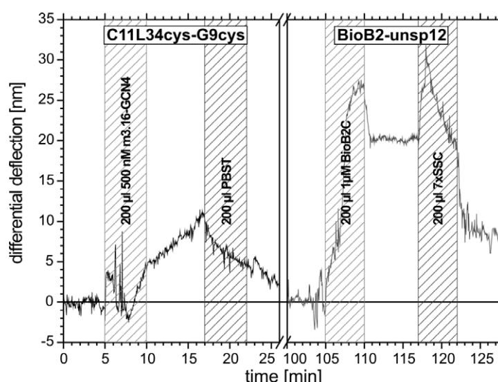
Figure 2. Differential signals upon sequential injections of 500 nM antigen m3.16-GCN4 at 5 min. and 1 \mu M complement oligonucleotide BioB2C at 105 min. 200 \mu l of analyte are injected at a flow rate of 40 \mu l/min. A deflection of 5 to 10 nm is recorded for the antigen binding and a signal of 20 nm is measured for the hybridization of the DNA complement. Cantilevers are washed after 17 min. with 200 \mu l PBST and at 117 min. with 200 \mu l 7xSSC.
