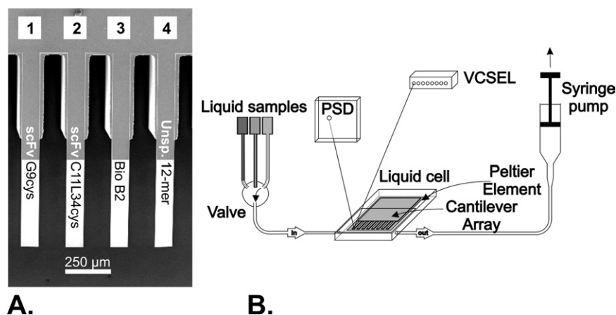
Figure 1A. Cantilever array showing 4 cantilevers functionalized with cystein modified single-chain antibody fragments, scFv G9cys used as reference, scFv C11L34cys probe, thiolated oligonucleotide BioB2 probe, and Unsp. 12-mer thiolated oligonucleotide used as reference. B. Device setup for measuring cantilever responses upon biomolecular interaction. A cantilever array is placed inside a liquid filled cell, which is on top of a peltier element. A laser beam is deflected at the end of a cantilever and its position is detected with a position sensitive detector (PSD) to measure cantilever bending. Target solutions or buffer are delivered by a syringe pump. Different analytes or buffers can be selected with a many fold valve. The whole setup is put in a temperature controlled box.
